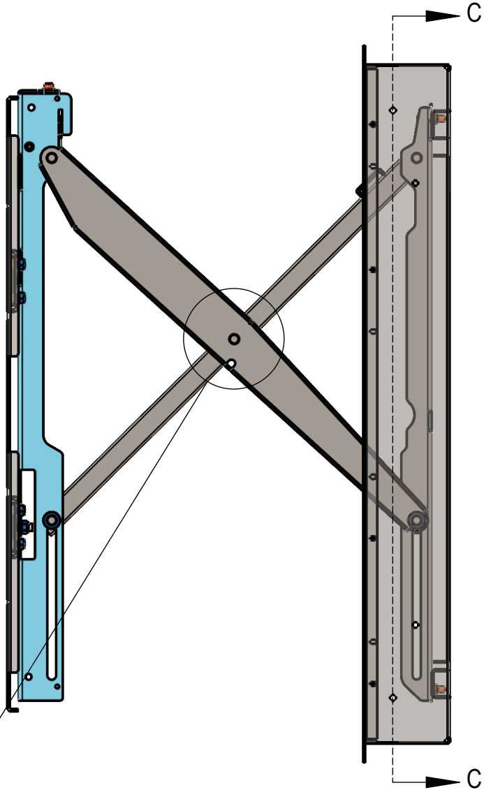
SIDE VIEW OPEN POSITION
