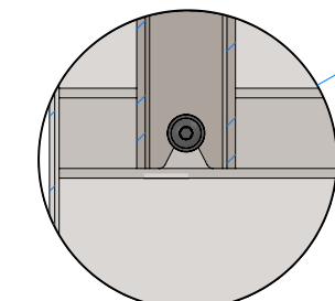
DETAIL E SCALE 1:3
