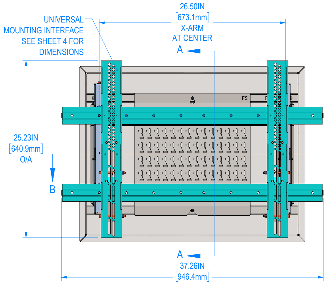
FRONT VIEW
