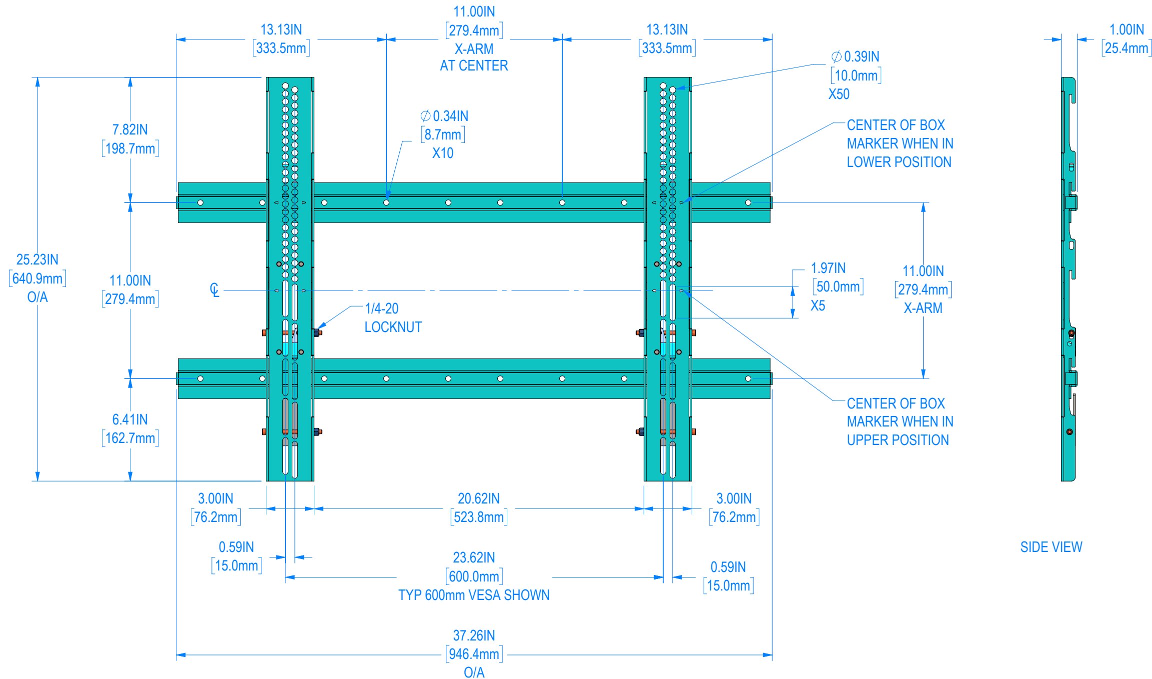
FRONT VIEW
