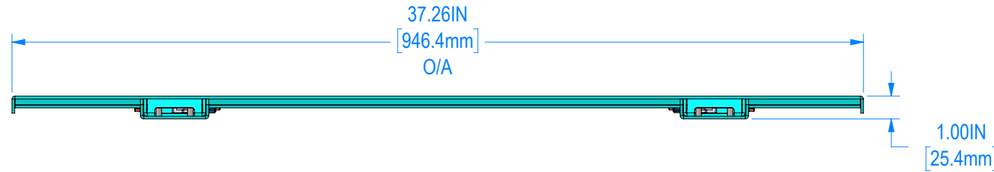
FRONT VIEW
