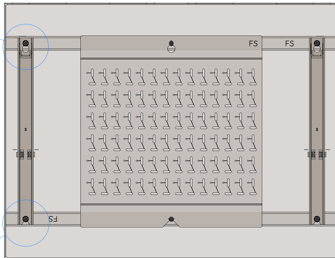
SECTION C-C
