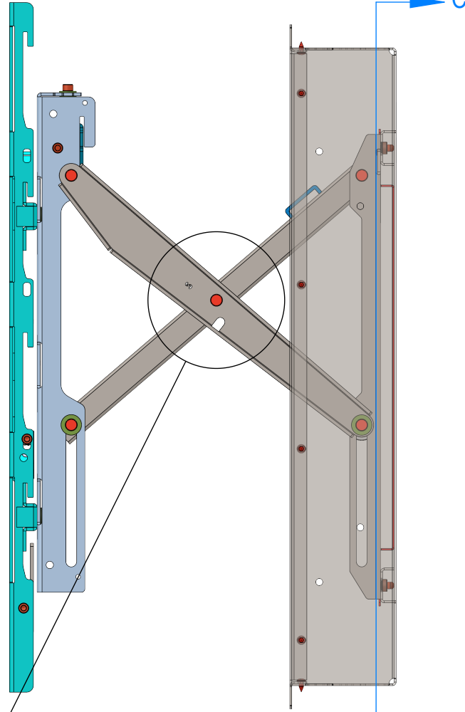
SIDE VIEW OPEN POSITION
