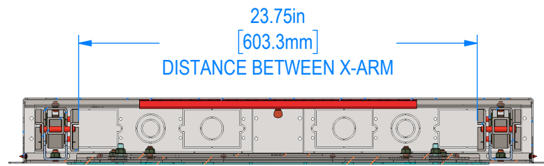
SECTION B-B
