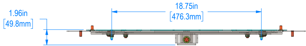
TOP VIEW
