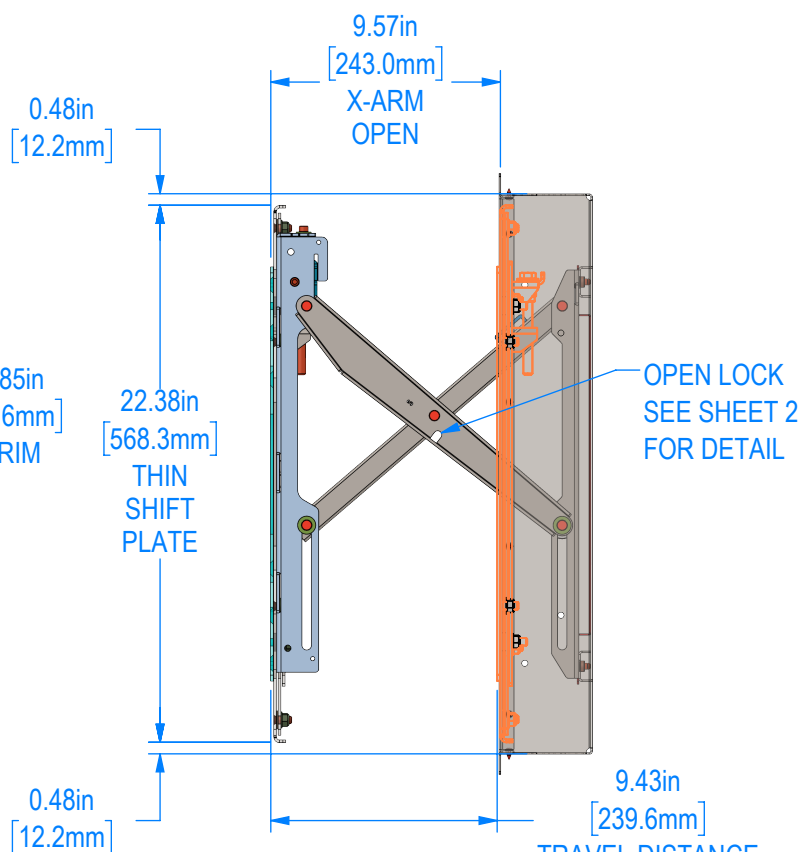
X-ARM OPEN
