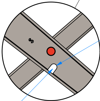
DETAIL F SCALE 1 : 3
