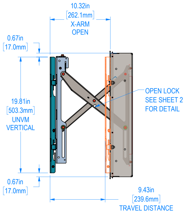
X-ARM OPEN
