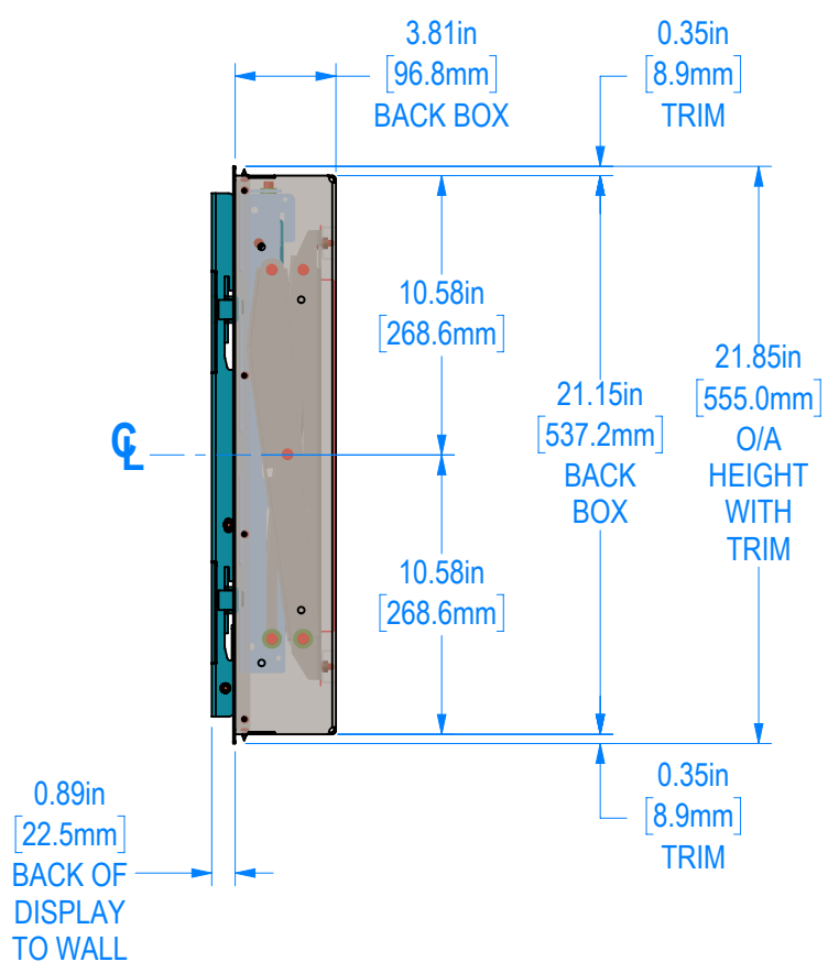
SIDE VIEW
