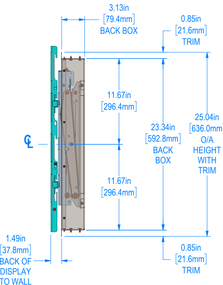
SIDE VIEW
