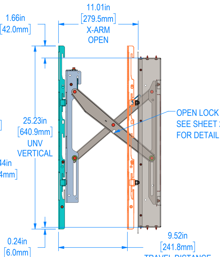
X-ARM OPEN
