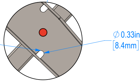
DETAIL D SCALE 1 : 3
