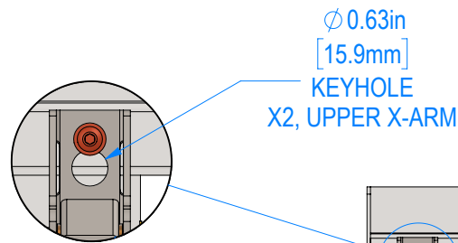
DETAIL H SCALE 1 : 3
