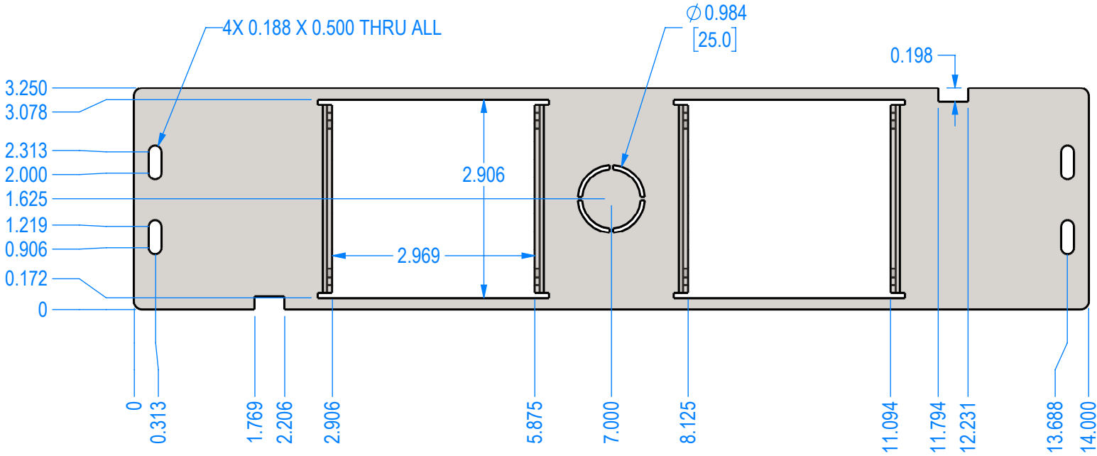
TOP VIEW
