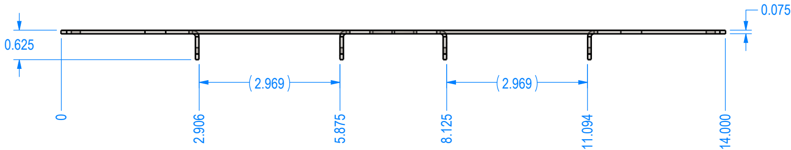
FRONT VIEW
