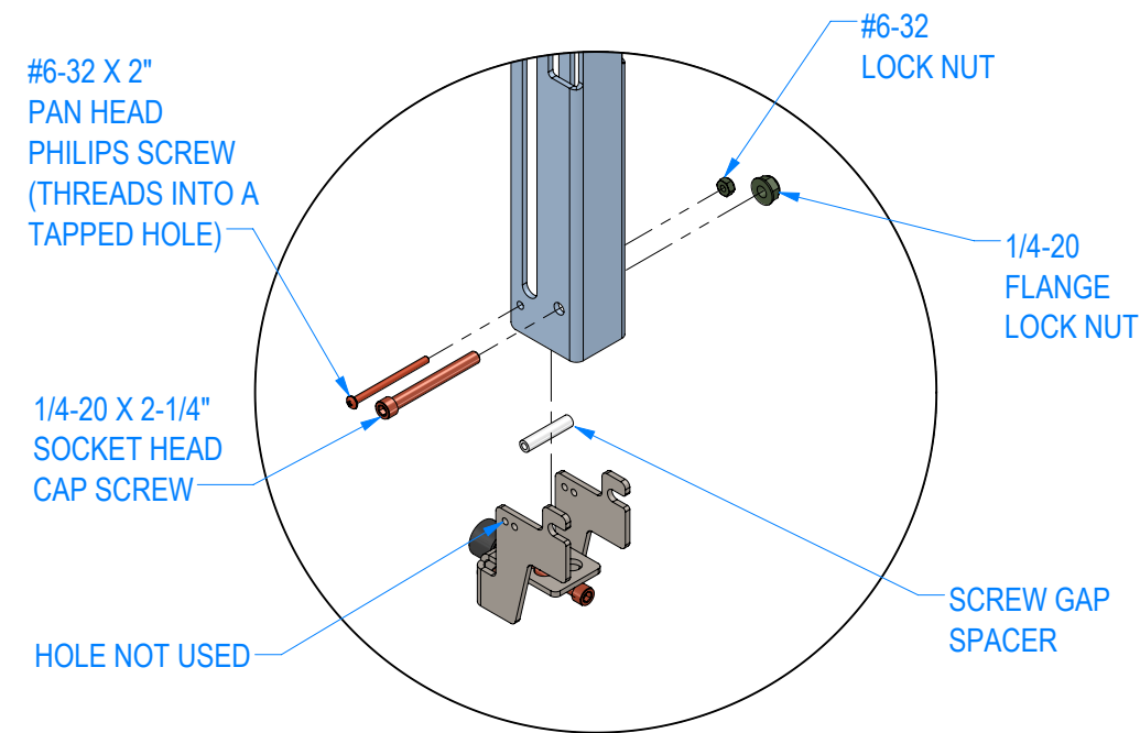
DETAIL H BOTTOM RIGHT BRKT SCALE 1 : 4
