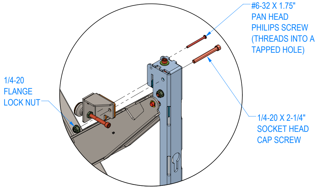
DETAIL G TOP RIGHT BRKT SCALE 1 : 4
