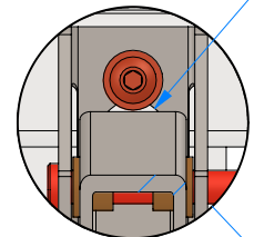
DETAIL K SCALE 1 : 2
