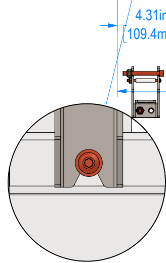
DETAIL H SCALE 1 : 2
