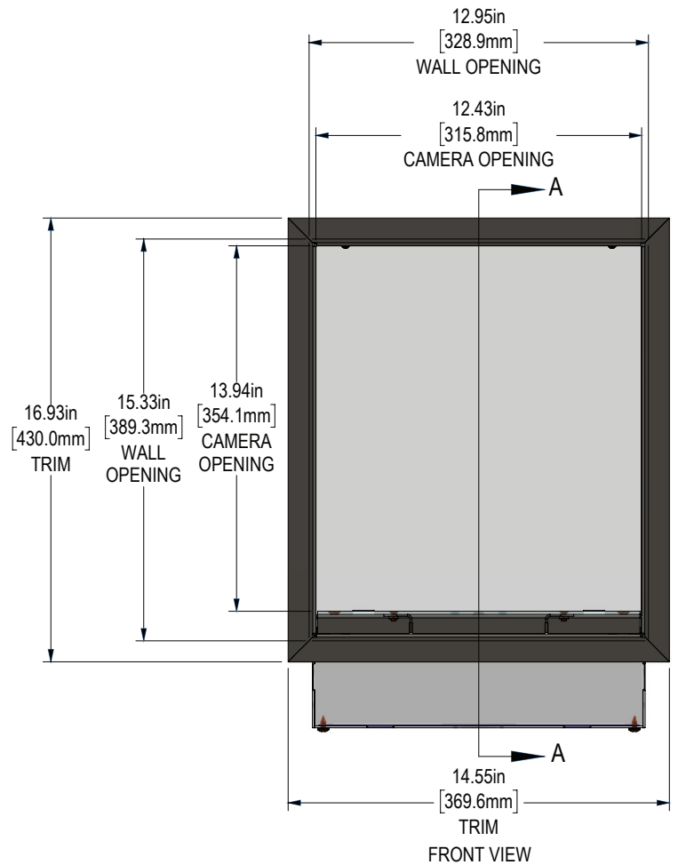
FRONT VIEW
